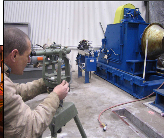
▲ Optical Alignment
