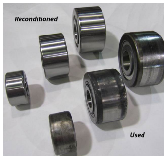
▲ Bearing reconditioning
