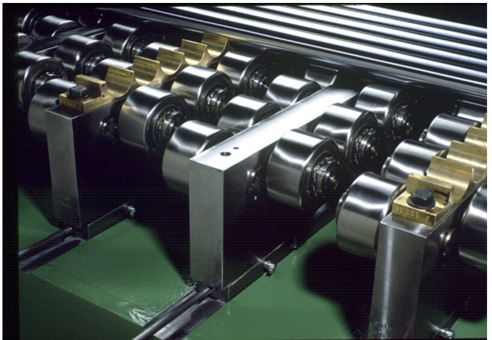
▲ Back-up supports with pins
